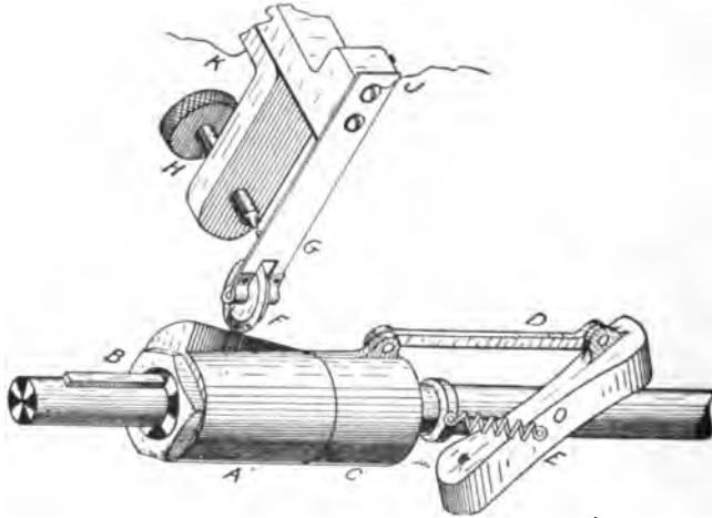
FIG. 406.—The Sliding Cam Ignition Governor of the "Packard" Carriages. A is a sleeve sliding on a feather, B, on the rotating shaft, being connected by link, D, to the governor weight, E, so that the throw of the cam, F, may be varied from maximum to zero, as the speed of the motor increases. Cam, F, bears upon the roller carried on the end of the vibrating leaf spring, G, modifying the electrical contact between the terminals, J and K, according to the throw of the cam and the adjustment of the screw, H.
